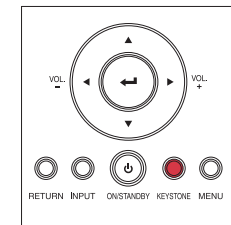
Control panel
